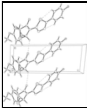
Fig. 2. A packing diagram for (I). Dashed lines indicate intramolecular C—H...S and C—H...N, and intermolecular C—H...O hydrogen bonding interactions.
