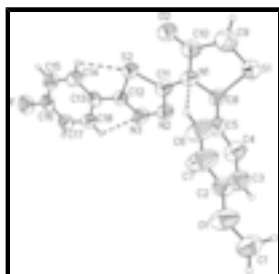
Fig. 1. A view of the molecular structure of (I). Displacement ellipsoids are drawn at the 50% probability level. Dashed lines indicate intramolecular C—H···S and C—H···N hydrogen bonding interactions.
